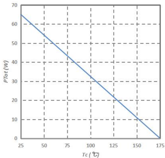
Fig.6-Power Derating
