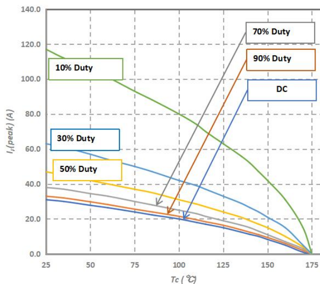
Fig.7-Current Derating
